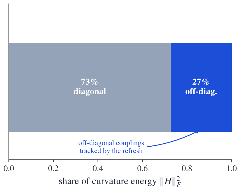
(b) A quarter of the curvature is off-diagonal
