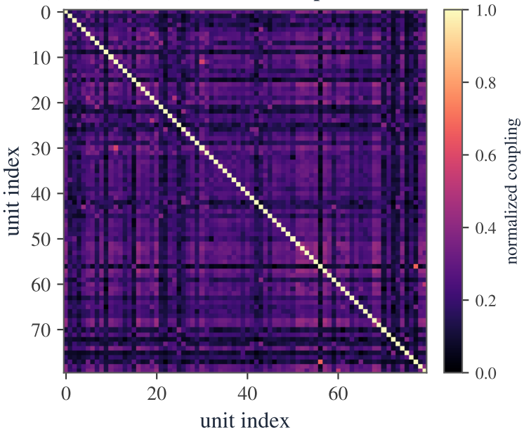
(a) Fisher curvature couples units
